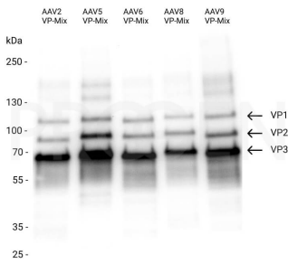
AAV8 VP1, recombinant protein
